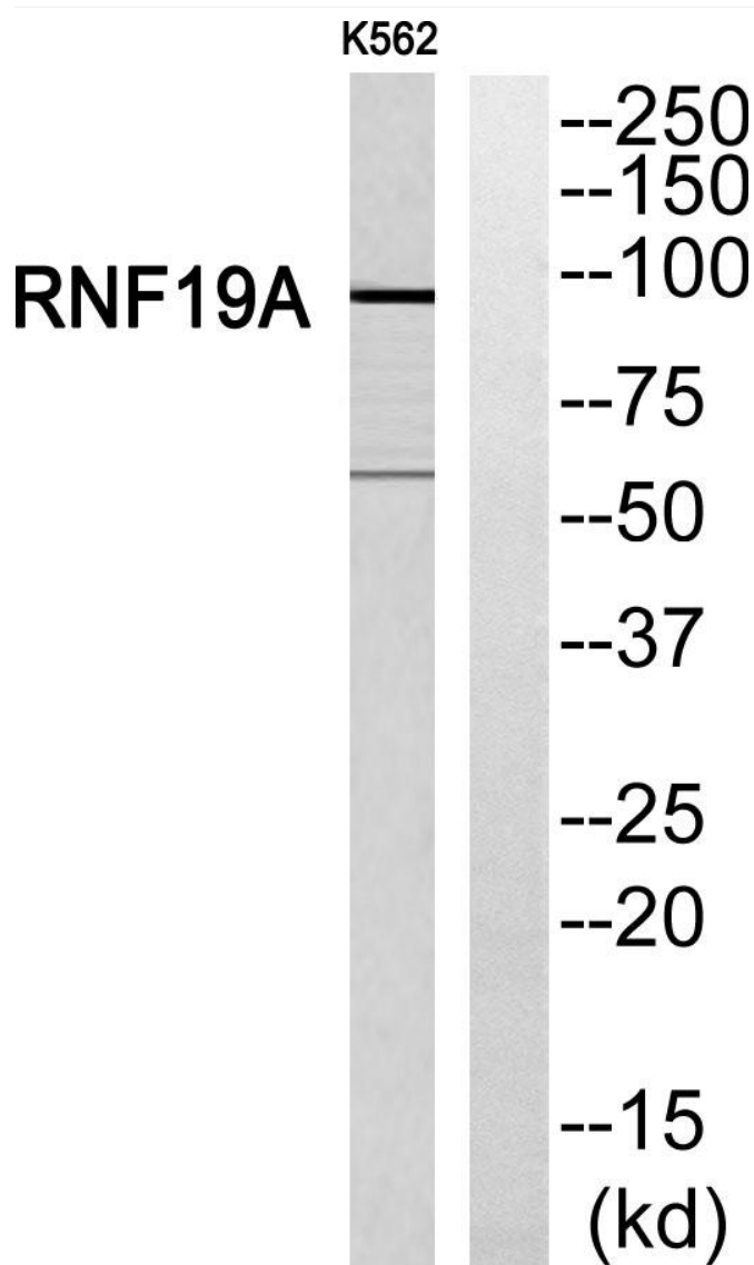
Western Blot analysis of various cells using Dorfin Monoclonal Antibody
