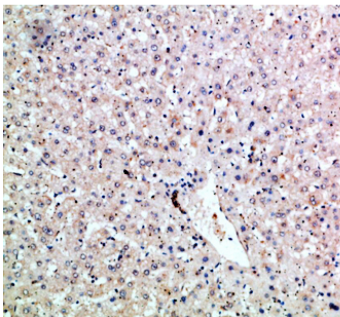
Immunohistochemical analysis of paraffin-embedded human-liver, antibody was diluted at 1:200
