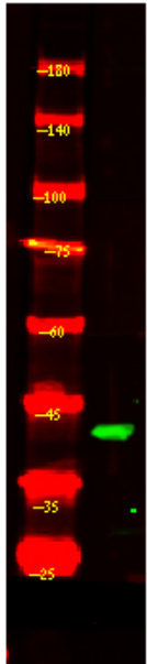
actin
