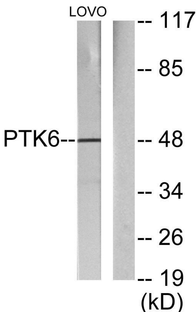
Western Blot analysis of various cells using Brk Monoclonal Antibody
