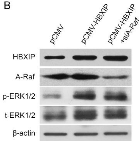
Western Blot analysis of various cells using A-Raf Monoclonal Antibody
