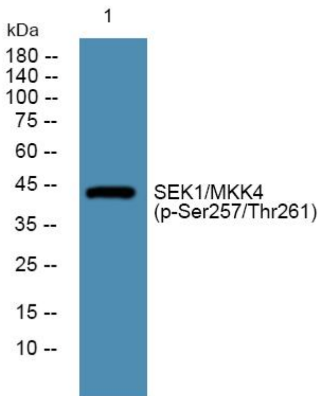
Western Blot analysis of various cells using SEK1/MKK4 (phospho-Ser257/Thr261) mouse mAb
