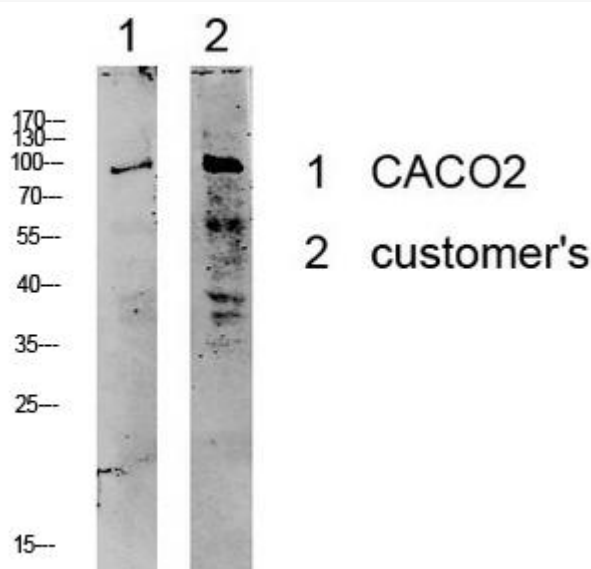
Western Blot analysis of various cells using Kv2.1/KCNB1 Monoclonal Antibody
